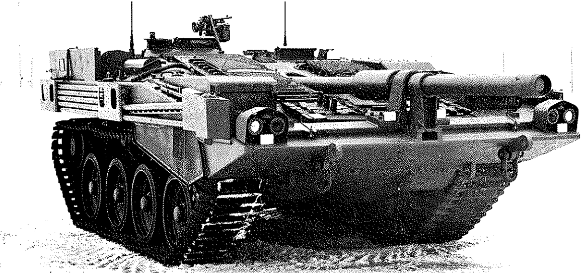
S-tank Type B with flotation equipment.
