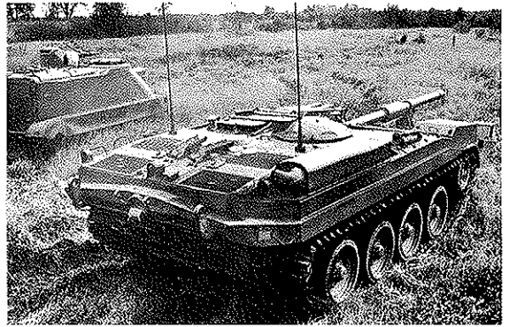
Rear view of an S-tank pre-production model which shows the location of the radiator louvres.
