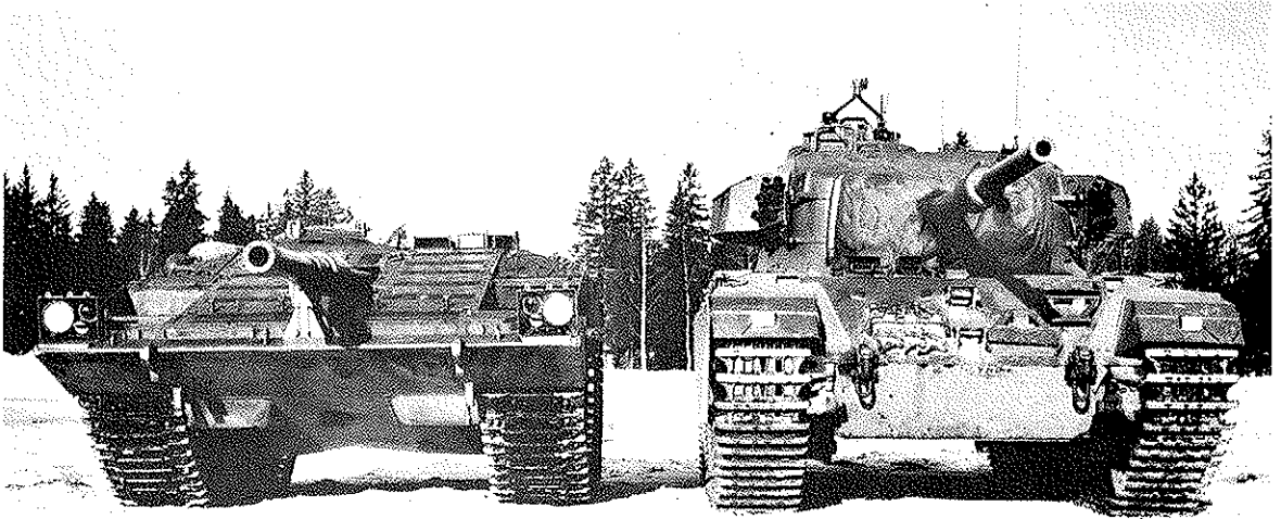
S-tank, left, compared with a conventional, turreted Centurion tank.
