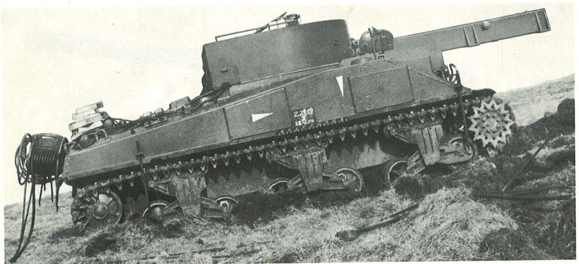
Sherman medium tank chassis with an internal "crowbar" steering system.
