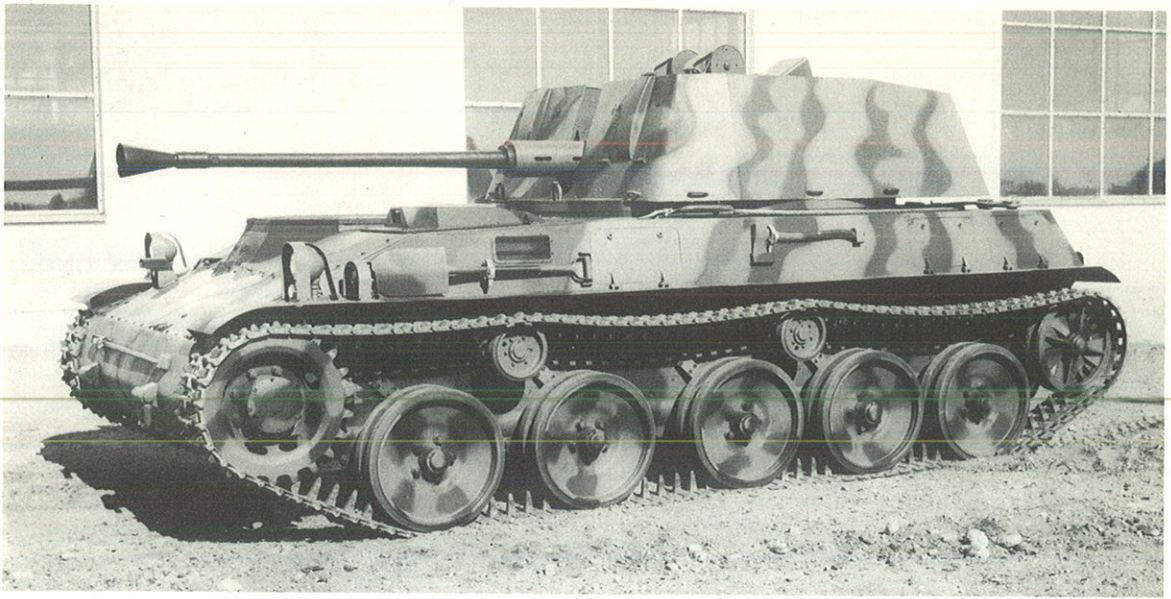
Lkv 42, an experimental 40-mm. self-propelled anti-aircraft gun with an adjustable suspension built by Bofors in 1954.
