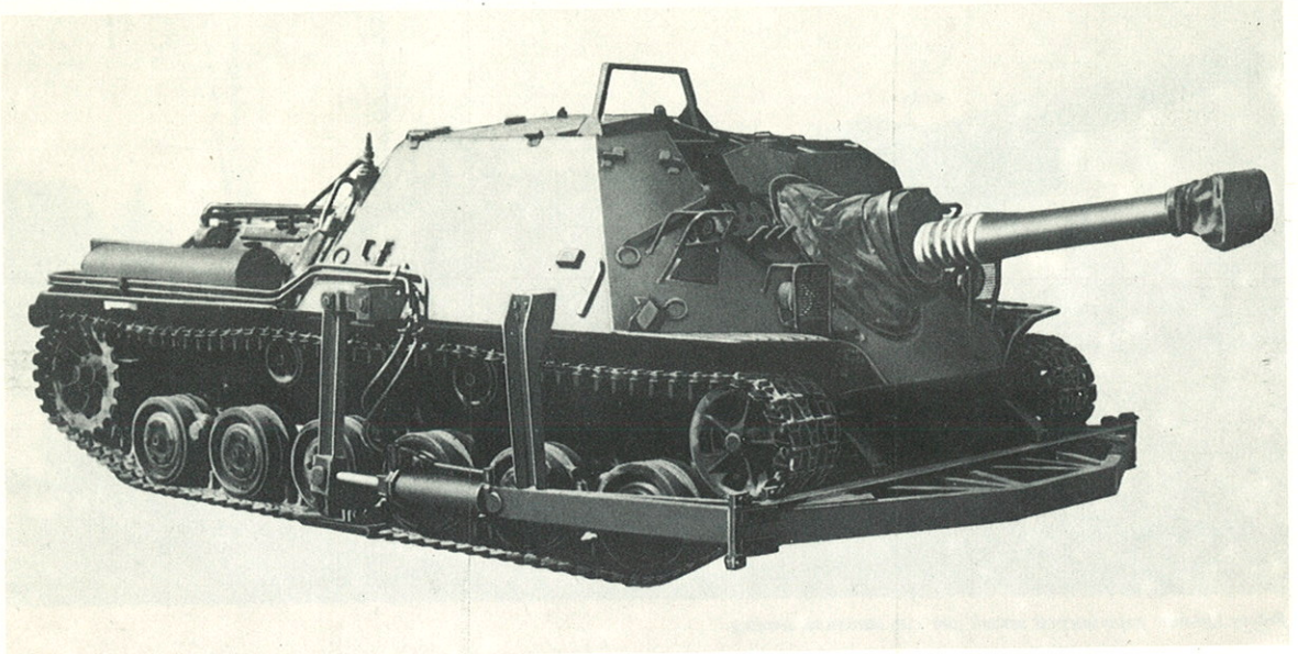
IKV 103 assault gun with an experimental, external "crowbar" steering system.
