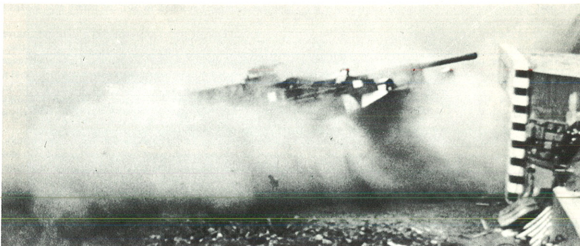
An S-tank exposed to the shock wave of a simulated nuclear explosion.
