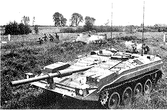
S-tank pre-production model with the original, domed commander's cupola.
