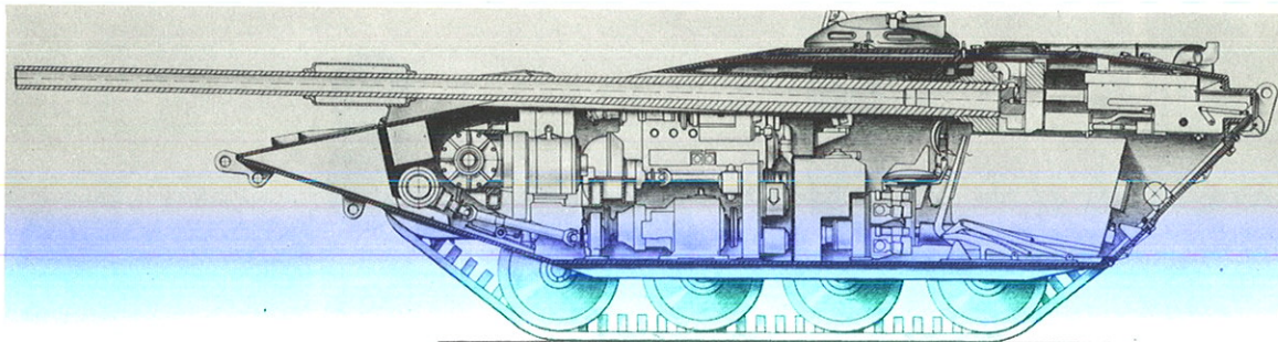
Sectioned drawing of the S-tank in prototype form which shows the forward location of the engines and transmission and the rear location of the ammunition magazine.
