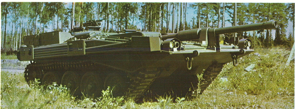
S - tank Type B
