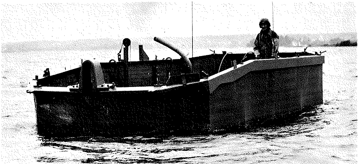
S-tank swimming with the aid of its flotation screen.
