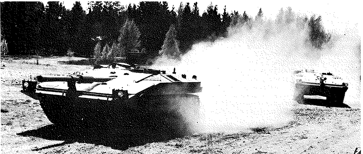
Pre-production models of the S-tank during trials: note the absence of the machine-gun boxes.
