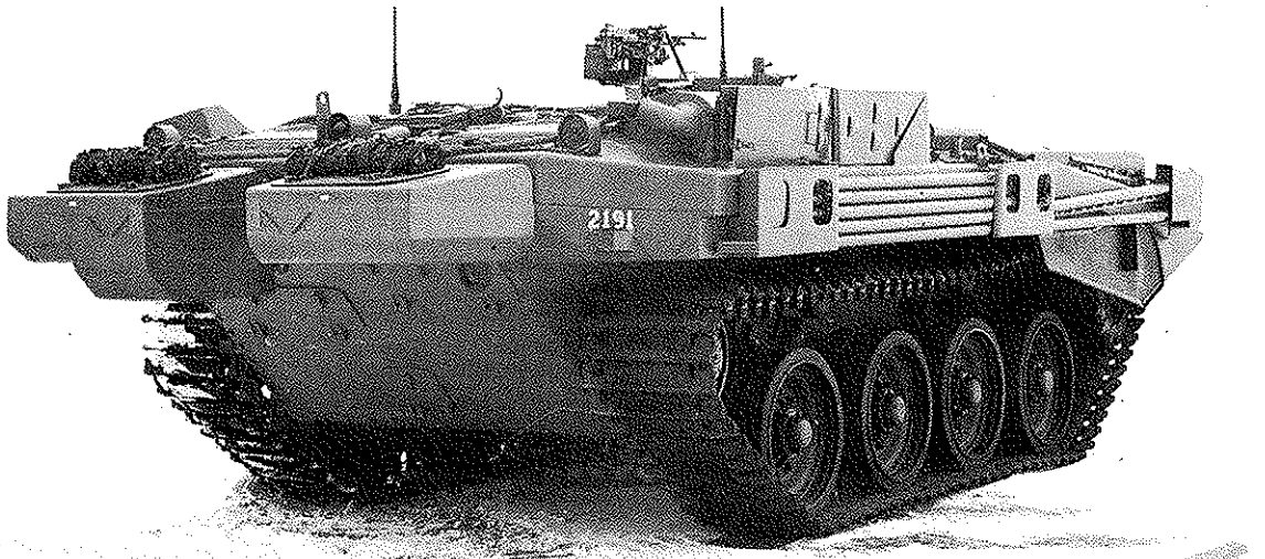
Rear view of an S-tank Type B with flotation equipment.
