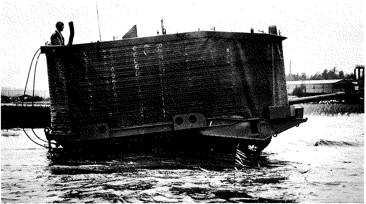
S-tank coming ashore with its flotation screen erected.
