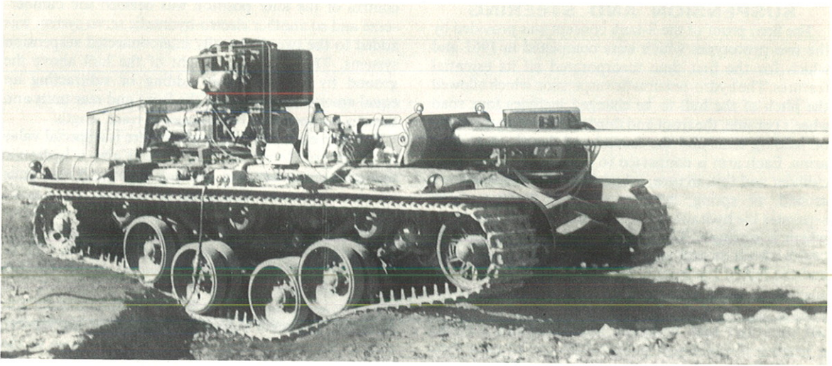
Test rig based on the KRV chassis fitted with a 83.4-mm. 20-pounder of the Centurion.
