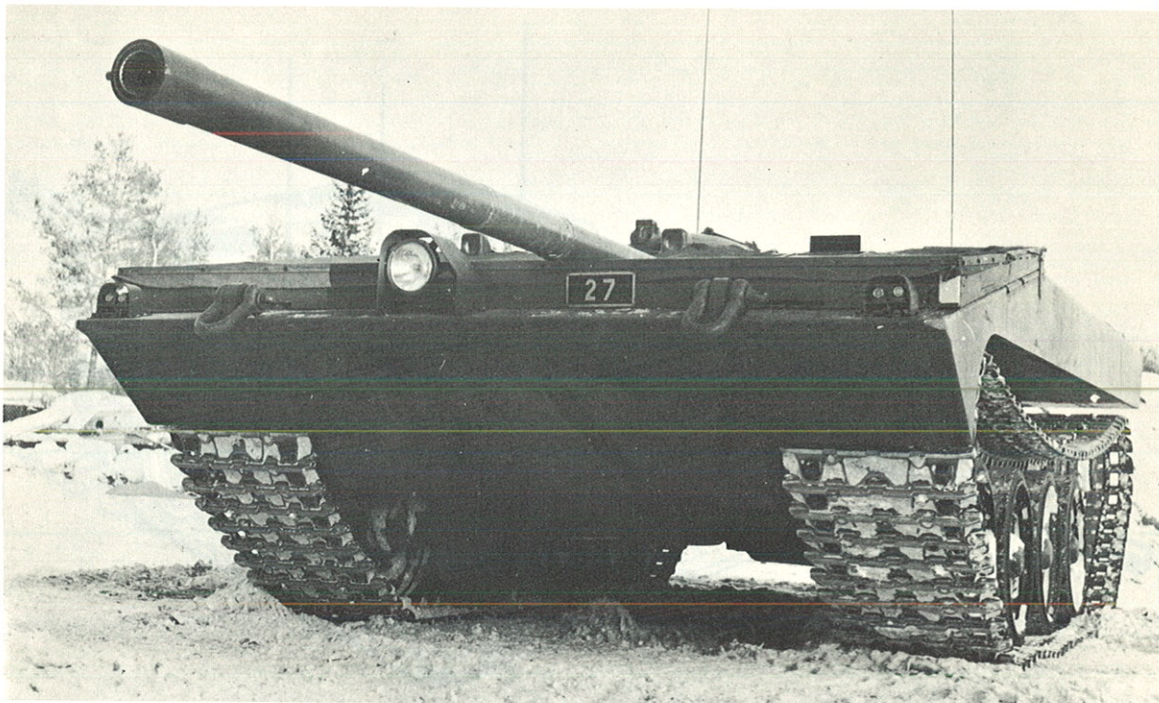
S-tank prototype with the original all-steel track.
